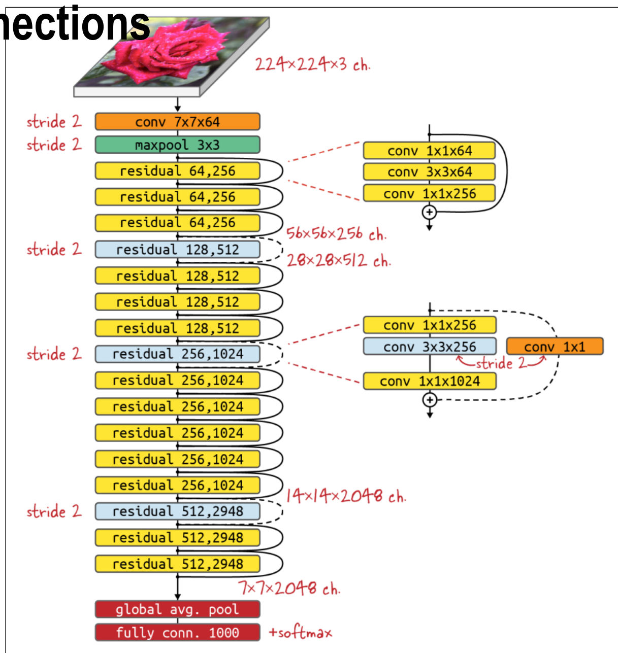
The ResNet50 architecture. Residual blocks with a stride of 2 have a skip connection implemented using a 1 \times 1 convolution (dotted line). The ResNet 101 architecture is similar, with the “residual 256, 1,024” block repeated 23 times instead of 6.
