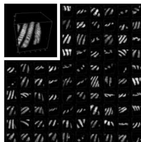
FractureMNIST3D
