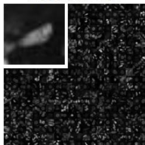
TissueMNIST
