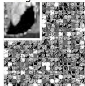
OrganCMNIST
