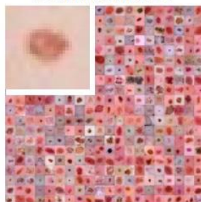
DermaMNIST
