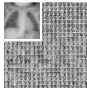
PneumoniaMNIST
