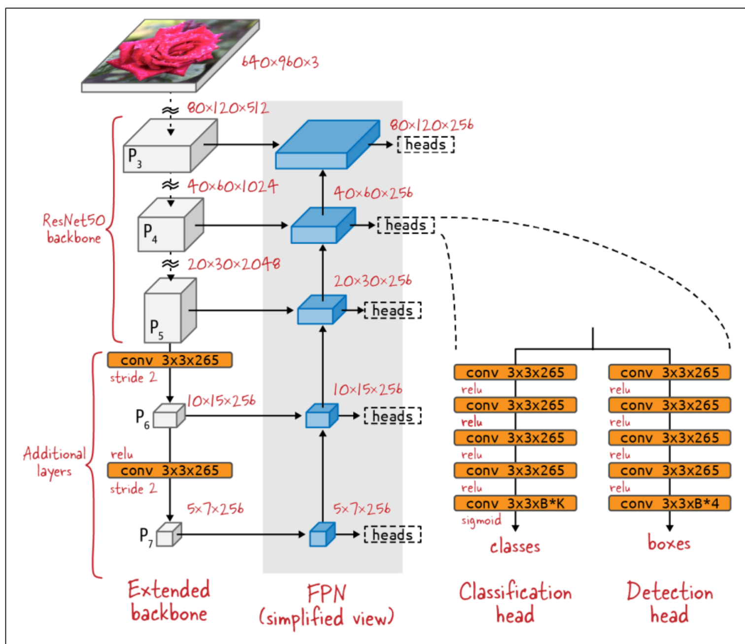
Complete view of the RetinaNet architecture. K is the number of target classes. B is the number of anchor boxes at each position, which is nine in RetinaNet.
